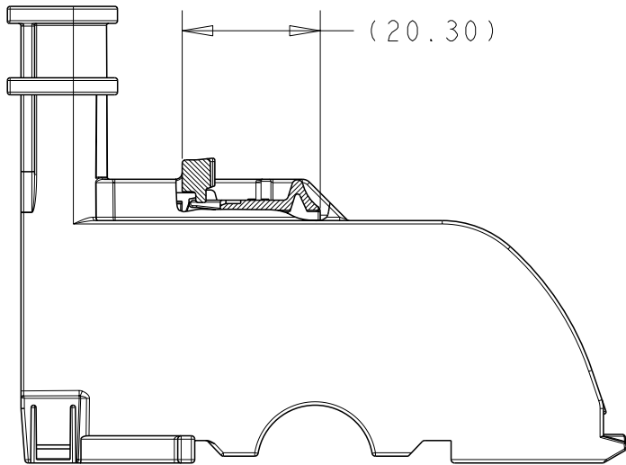
CPA IN OPEN POSITION SECTION D-D
